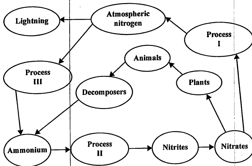
Figure 1. The nitrogen cycle
